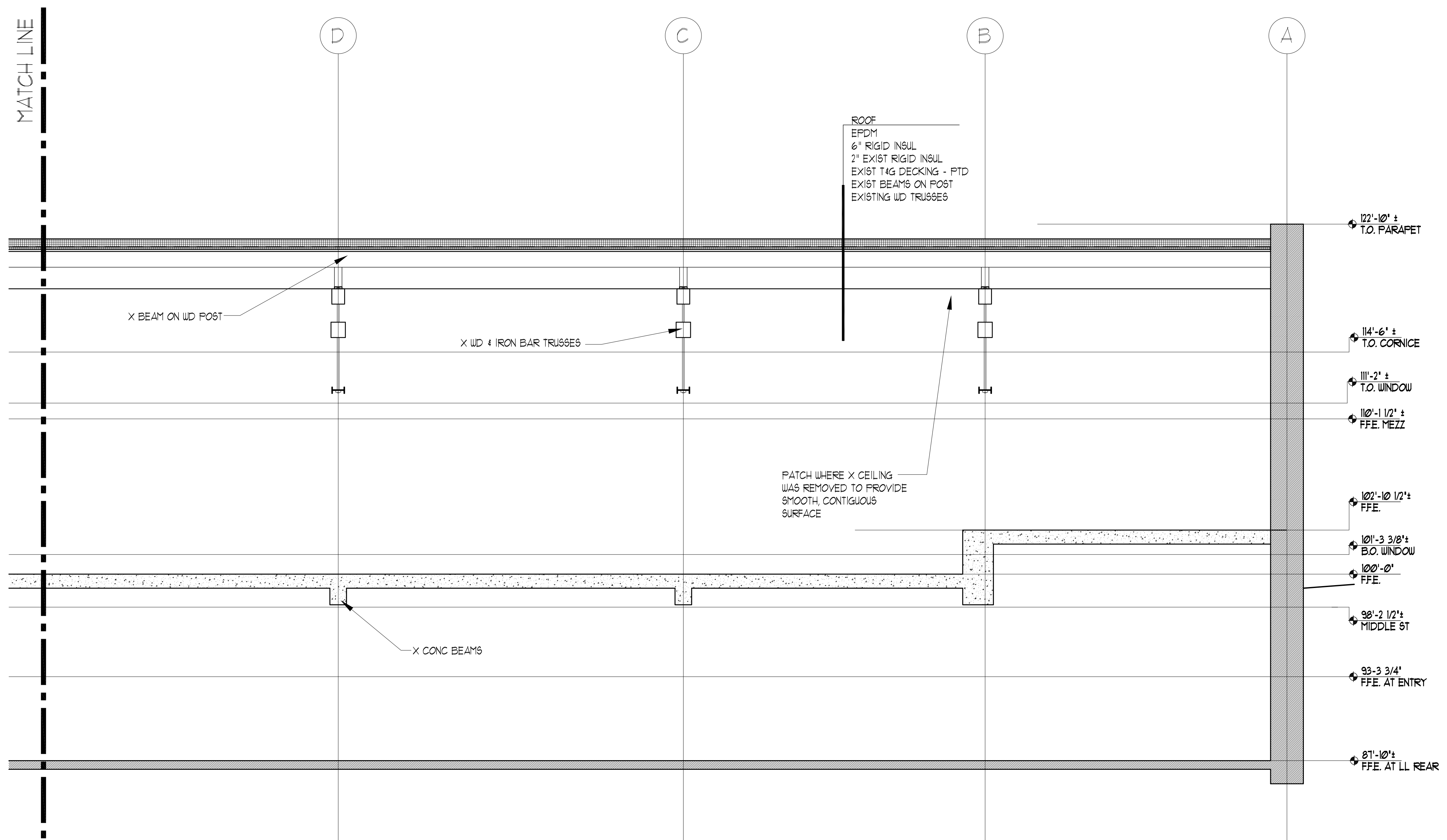
BUILDING SECTION A11 A3.4 SCALE: 1/4" = 1'-0"
